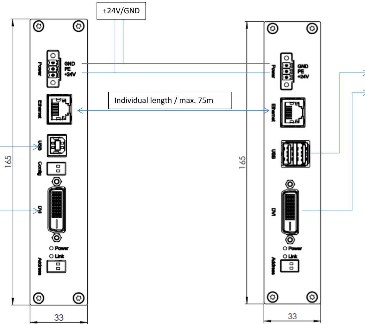
C-Link Transmitter
